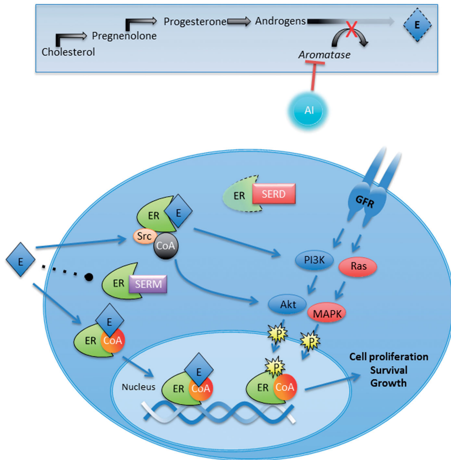
Figure 1. The role of oestrogen in endocrine-mediated cell proliferation and survival. Upon oestrogen (E) binding, the oestrogen receptor (ER) recruits co-activator complexes (CoA) and localises on specific DNA sites to initiate the transcription of growth factor genes as well as receptor tyrosine kinases that go on to mediate proliferation, survival and growth. Cytoplasmic ER can also bind to receptor tyrosine kinases in response to oestrogen stimulation resulting in activation of downstream kinase pathways. Aromatase inhibitors act by inhibiting the aromatase enzyme. This enzyme is responsible for the conversion of androgens into oestrogens. This results in the decreased levels of oestrogen. Selective oestrogen receptor modulators/degraders (SERM and SERD respectively) target the ER. SERMs bind and antagonise the ER thereby preventing oestrogen-mediated signalling. SERDs also bind to ERs and inhibits dimerisation, thus it is unable to form complexes or function correctly and consequently degraded.
