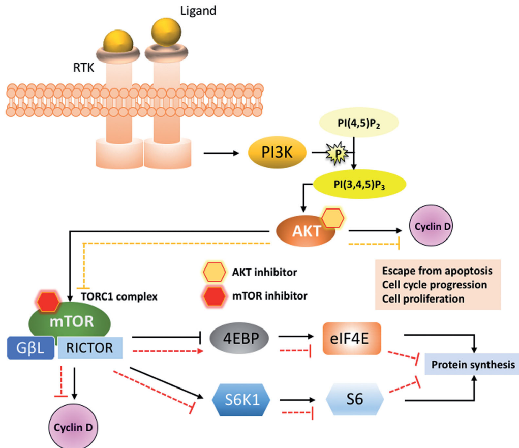
Figure 3. Schematic overview of the PI3K/AKT/mTOR pathway. Upon ligand binding, the receptor tyrosine kinase (RTK) activates PI3K which in turn phosphorylates PI(4,5)P 2 and converts it to PI(3,4,5)P 3 . PI(3,4,5)P 3 activates AKT by phosphorylating its serine-308 and threonine-473 residues. Once activated, AKT stimulates a cascade of downstream signals, including the nuclear accumulation of cyclin D, that promote cellular growth, survival and proliferation. Phosphorylated AKT also activates mTOR which forms the TORC1 complex. mTOR then targets downstream signalling molecules that result in the synthesis of proteins that play a role in maintaining survival and promoting proliferation. Genetic mutations lead to constitutive activation of the PI3K/AKT/mTOR pathway and are common in BC. Thus, the development of inhibitors (yellow and red hexagons) have allowed for the disruption of these pathways in an attempt to impede aberrant cell behaviour as shown by the dashed lines.
