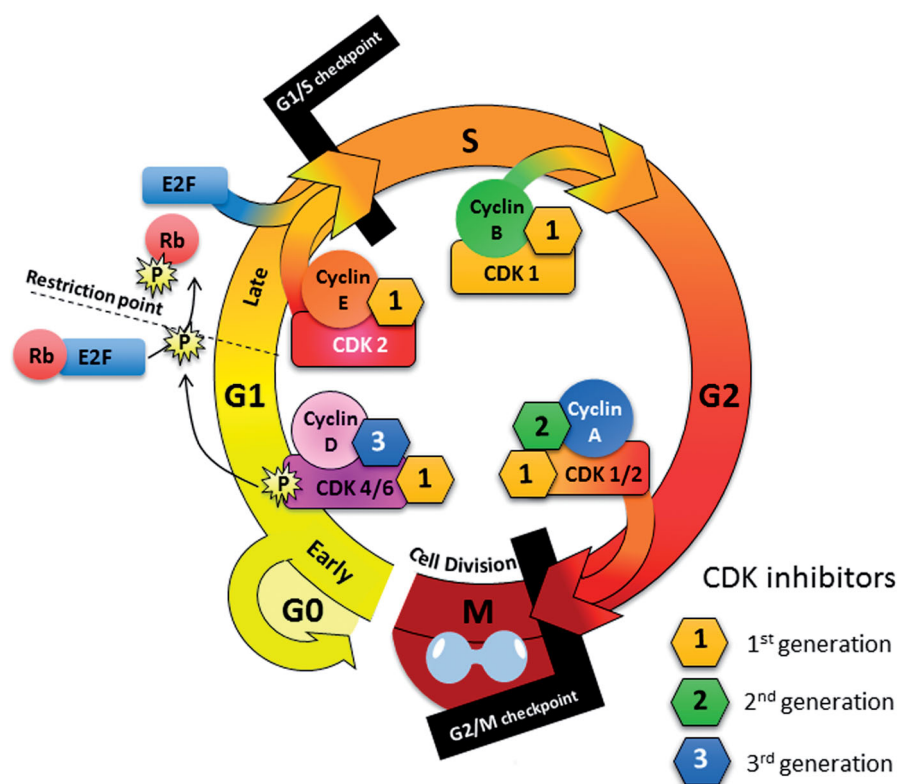
Figure 2. Cell cycle phases. The cell cycle progresses through a number of phases in order to commence with a successful division process. Cells prepare for cell division by using the gap phases to duplicate proteins, organelles and DNA. During the first gap phase, G1, the cell assesses the internal and external environments to determine its ability to progress through to the next phase. If conditions are unfavourable, the cell will leave the cell cycle and remain in a resting phase, G0, where it will remain dormant until stimulation from external factors. If, however, the conditions are favourable, the cell will progress into the S phase where DNA synthesis occurs. The second gap phase, G2, commences to allow for DNA replication. Provided that there have been no delays, damage or inhibition at previous stages, the cell will continue into the final stage of division, the mitotic (M) phase, where mitosis and cytokinesis are initiated. Passage from one phase to another is tightly regulated by checkpoints. These ensure that essential cheques have been undertaken in order for the cell to correctly reproduce its genetic material with no errors that may result in the death of the cell, or in the case of cancer, aberrant cell proliferation. Under normal, resting, conditions, Rb exists in an inhibitory complex with E2F and other corepressors. If cell division is initiated, cyclin/CDK complexes are activated to phosphorylate RB, lifting its inhibitory function and allowing transcription of cell cycle genes. CDK inhibitors target CDKs and inhibit their function, this results in Rb remaining in an unphosphorylated state and the cell remains in the resting phase.
