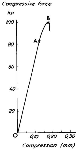
Figure 1. Force-compression diagram for compression tests on a bone specimen. From O to A the curve is approximately straight and the compression proportional to the applied force. The stress (compressive force/cross sectional area of the body) for the bone at A is the limit of proportionality ( kp/mm^2 ). The compression at rupture (B) is expressed as the percentage deformation of the original length of the body. The modulus of elasticity is the ratio of stress to strain, that is:
