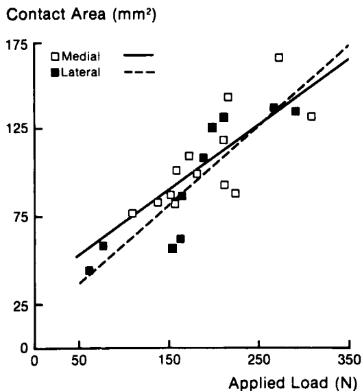
Figure 3A. Applied load (P) versus contact area (A) for chronic defects in medial and lateral compartments. There is a strong relationship between applied load and contact area. Linear regressions and correlation coefficients for the medial and lateral compartments, respectively, were
