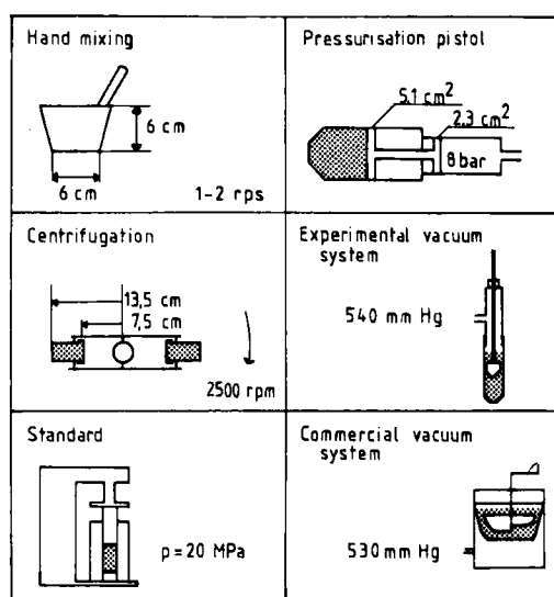
Figure 1. Specifications for the hand-mixing method (upper left), pressurization pistol (upper right), centrifuge (middle left), experimental vacuum system (middle right), pressure curing for the reference bars (lower left), and the commercial vacuum system (lower right).
