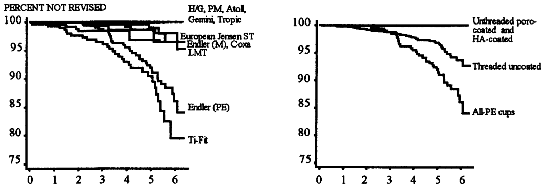
Figure 1. Prosthesis survival until revision for aseptic loosening of the cup. Total material of uncemented cups analyzed by type and by design characteristics.
