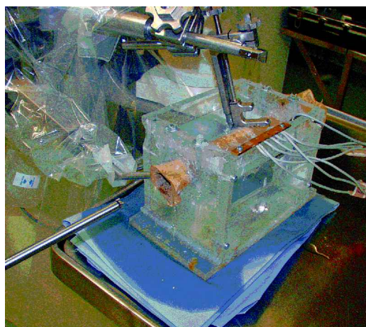
Figure 2. Water tank with cadaver bone mounted on the robot.
