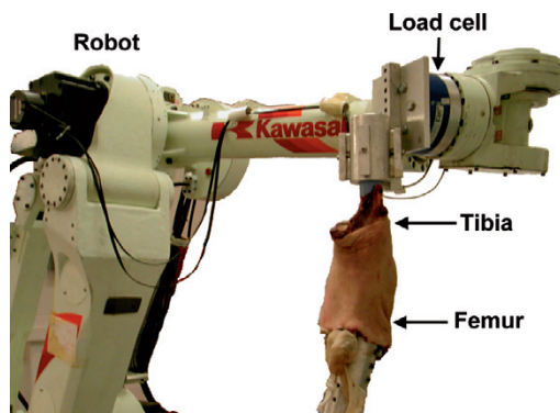
Figure 1. The robotic testing system with a knee specimen installed.
