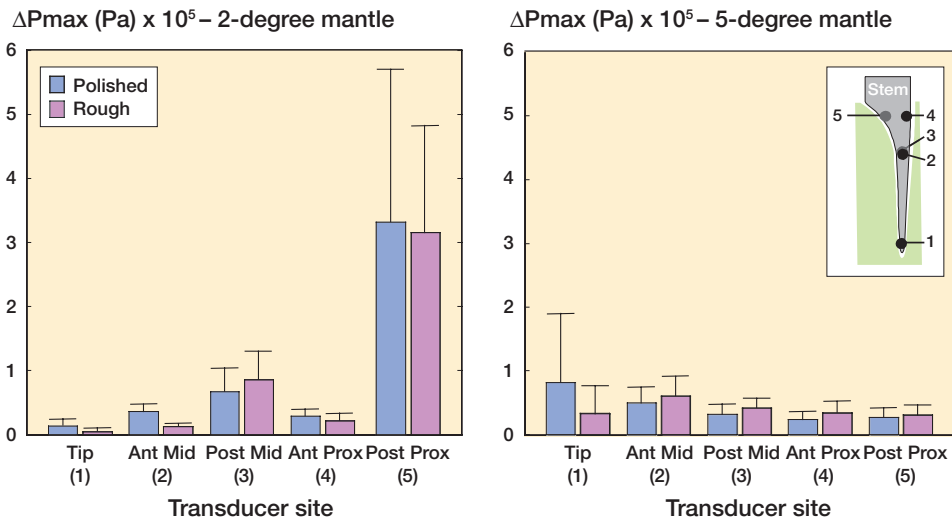
Figure 2. \Delta P_{\max} values (in Pa) recorded at each transducer site (see insert) for both rough and polished stems under combined physiological loading, in both the 2-degree and 5-degree mantles.
