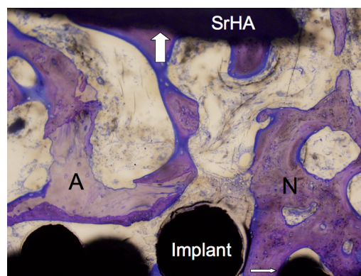
Figure 5. The implant-bone interface showing gap healing and ongrowth of bone onto the implant and SrHA. New bone (N), preserved allograft (A), ongrowth onto the implant (thin arrow), and ongrowth onto the SrHA (thick arrow). 10× objective.
