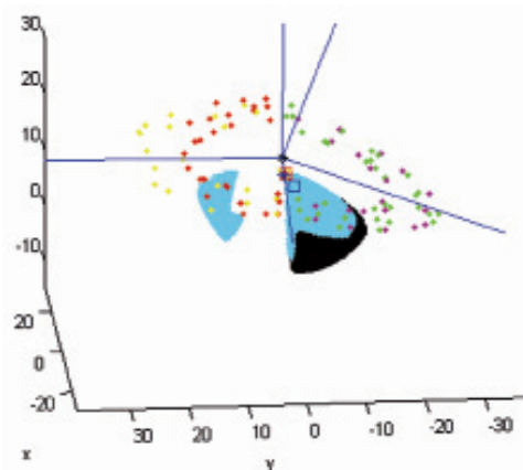
Figure 2. B. Example of CMM measurement. Digitized points on cup inner surface and planes, center points before and after wear (square hollow symbols), and coordinate axes (blue lines). Values are in mm.
